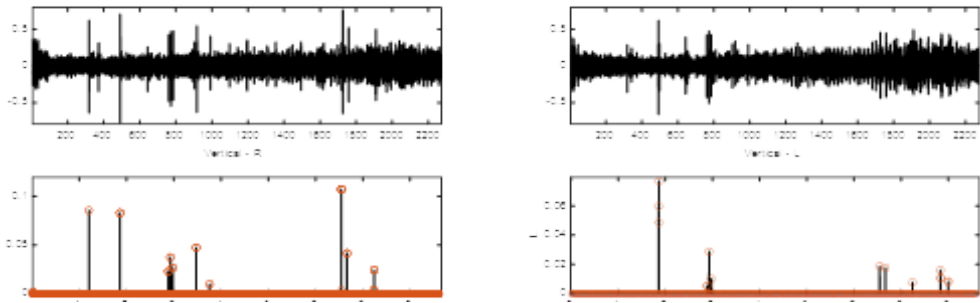
Figure 18-1 Example of a ABA measurement result. Upper graphs shows the raw acceleration signal with (y-axis in [g] and x-axis in meters). Lower graphs shows the detected anomalies for both rails (y-axis in relative intensity, x-axis in meters)
