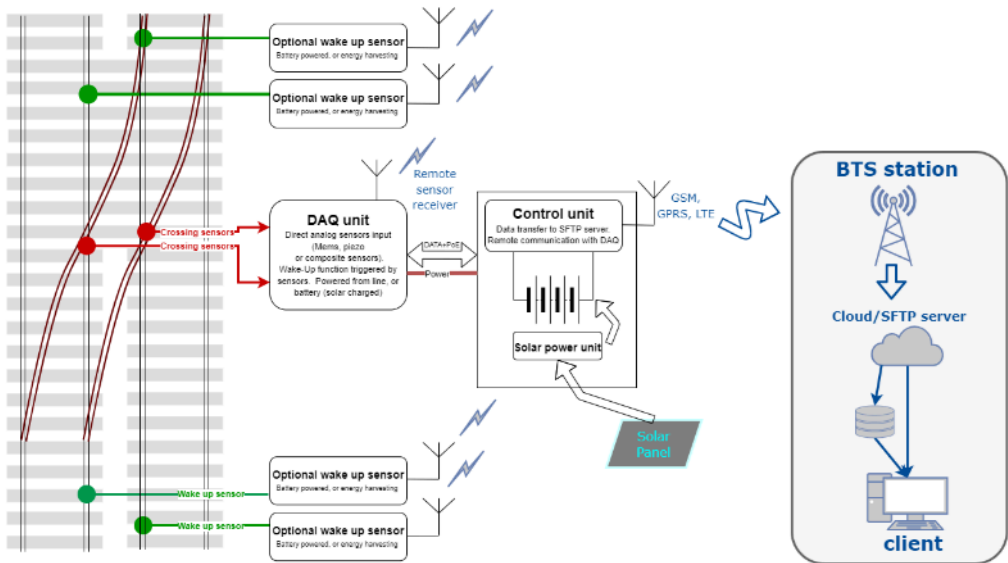
Figure 6-1 Data acquisition architecture
