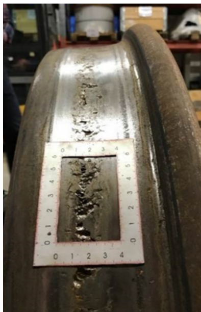
Figure 44-1 Wheel with severe rolling contact fatigue damage
