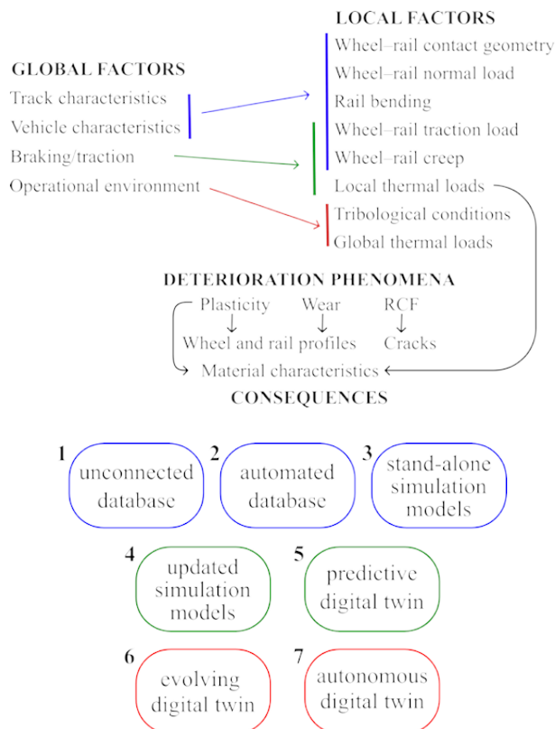
Figure 17-1 Top: Relations between some global operational conditions, local influencing factors, subsequent phenomena, and resulting consequences. Bottom: Evolution of "digital twins" from stand-alone databases and models (1–3), through models updated from measured data (4–5), to automatically updated digital twins (6–7)
